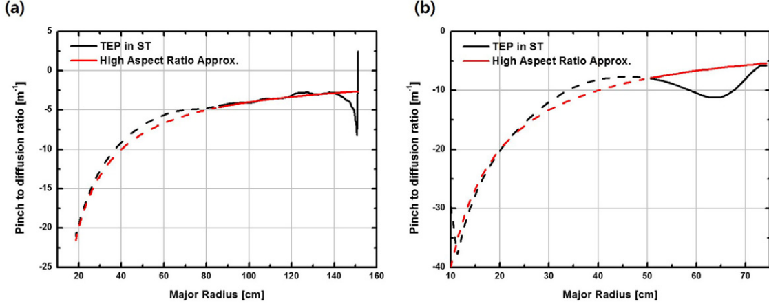
Figure 1. Pinch to diffusion ratio for typical equilibria of (a) NSTX ( \beta = 0.11 , A = 1.27 ) and (b) VEST ( \beta = 0.04 , A = 1.25 ). The black lines correspond to our new result in equation (14). The red lines are -4/R from [16]. Here, only the solid line part corresponding to the low field side of a given flux surface should be considered.
