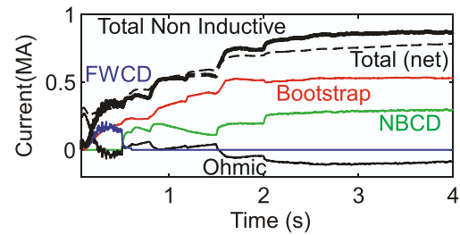
Figure 14. Fully non-inductive current scenario for a 1 T NSTX-U discharge as computed by TRANSP with the ISOLVER free boundary equilibrium solver.
