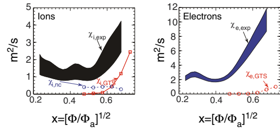
Figure 27. Comparison of experimental and GTS predicted thermal diffusivity for ions (left panel) and electrons (right panel). The experimental values of \chi_e and \chi_i were computed in TRANSP in interpretive mode, and the ion neoclassical value was computed using GTC-NEO. The abscissa is x = [\Phi/\Phi_a]^{1/2} , where \Phi/\Phi_a is the toroidal flux normalized to the value at the boundary.
