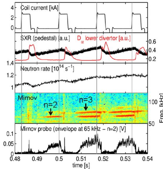
Figure 13. TAEs modulated by pulsed edge MPs.
