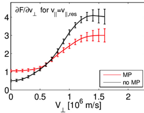
Figure 12. \partial F_{fast}/\partial v_{\perp} at the parallel resonant velocity as computed by TRANSP and SPIRAL with (red) and without (black) applied MPs.
