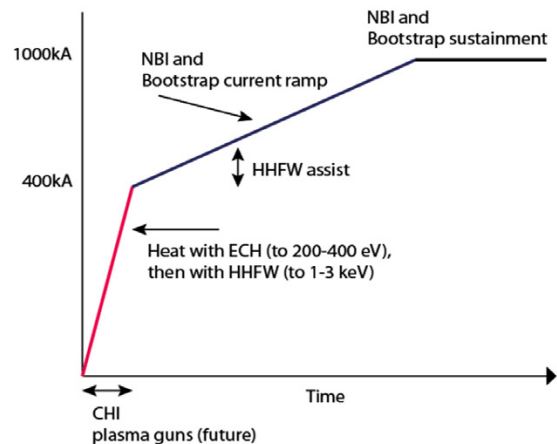
Figure 1. Strategy for fully non-inductive operation in NSTX-U.
