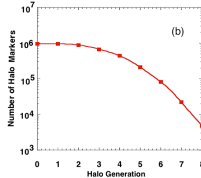
Figure 2. Schematic of the 3D halo neutral generation process (a) and a typical example of 3D halo generation evolution from the NUBEAM code (b).
