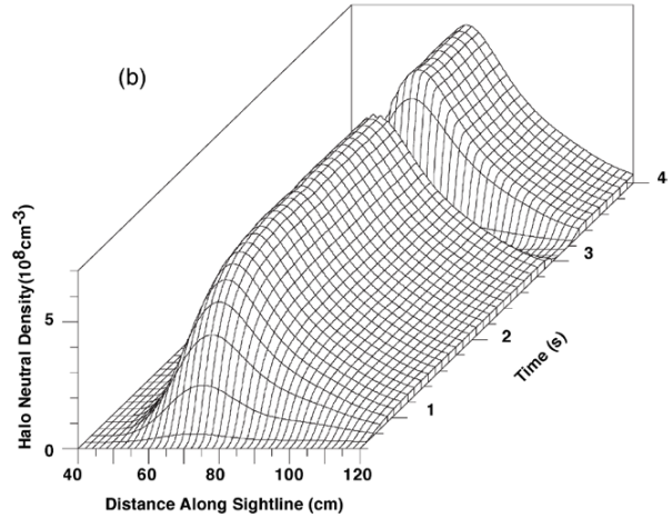
Figure 11. Injected beam neutral density (a) and halo neutral density (b) as a function of distance along the ssNPA sightline depicted in figure 4.
