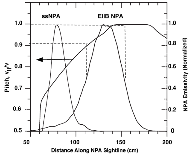
Figure 17. Comparison of particle pitch, v_{||}/v , for the ssNPA and E||B NPA emissivity distributions along the sightlines depicted in figure 4.
