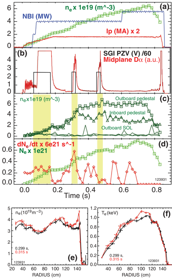
Fig. 13. Time traces of a representative SGI-2-fueled H-mode discharge: (a) plasma current I_p , NBI power, line-averaged density \bar{n}_e ; (b) midplane D_\alpha emission and SGI-2 valve control voltage; (c) electron density measured by the Thomson scattering system in the SOL and at the H-mode pedestal (inboard and outboard); (d) total electron inventory and its time derivative; (e) electron density profiles before and after the SGI-2 pulse; and (f) electron temperature profiles before and after the SGI-2 pulse.
