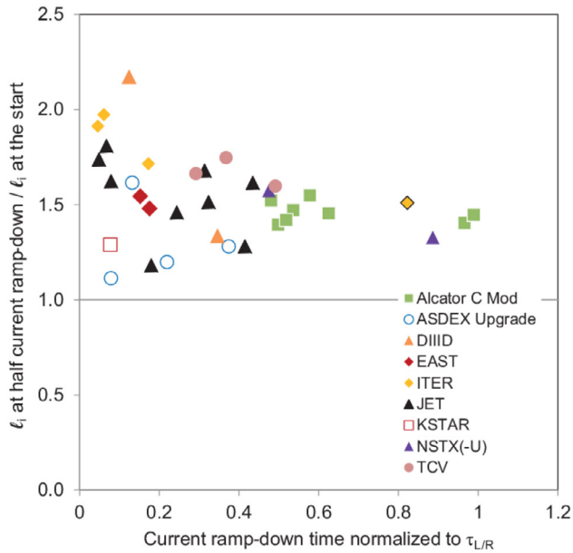
Figure 10. Existence diagram of the relative change in \ell_i over half the current ramp-down versus the ratio of the averaged current decay time and \tau_{LIR} .
