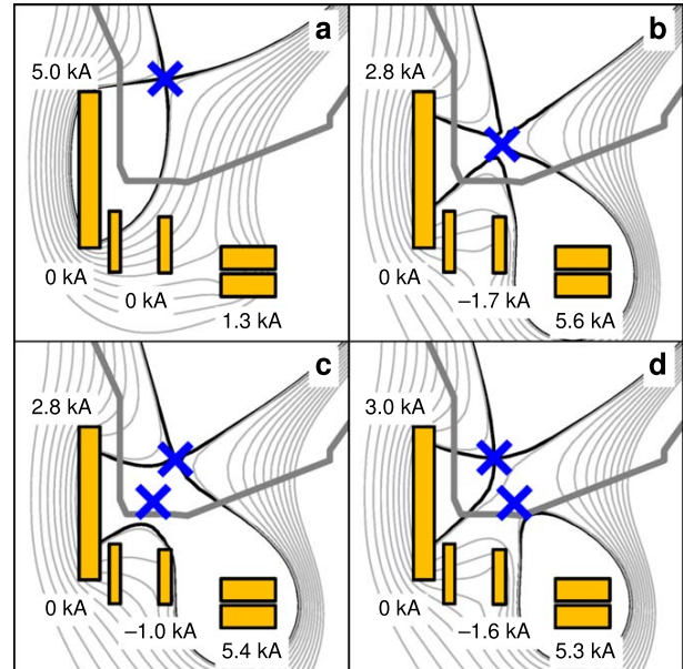
Figure 1. Several divertor configurations on NSTX-U as computed by a free-boundary equilibrium solver with I_p = 1 \text{ MA} , \beta_p = 1.0 , and I_i = 0.6 . Shown are (a) the standard single-null divertor, (b) the exact snowflake configuration with a second-order null, (c) the snowflake-plus configuration with a secondary null in the private flux region, and (d) the snowflake-minus configuration with a secondary null in the scrape-off layer. Also shown are the divertor coils (yellow) and coil currents for each configuration.
