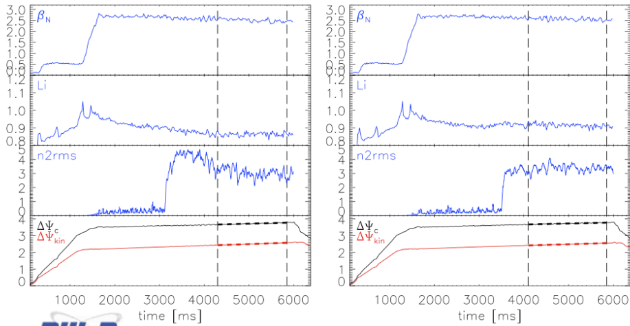
162894: counter-ECCD 3/2 mode destabilization
