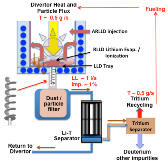
Fig. 1. A simplified schematic for the LL purification loop in a 1GW-e fusion power plant.
