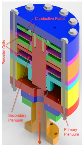
Fig. 1: Internal view of the NSTX-U double flyer plate MGI valve. Gas from the primary plenum is injected into the plasma discharge.
