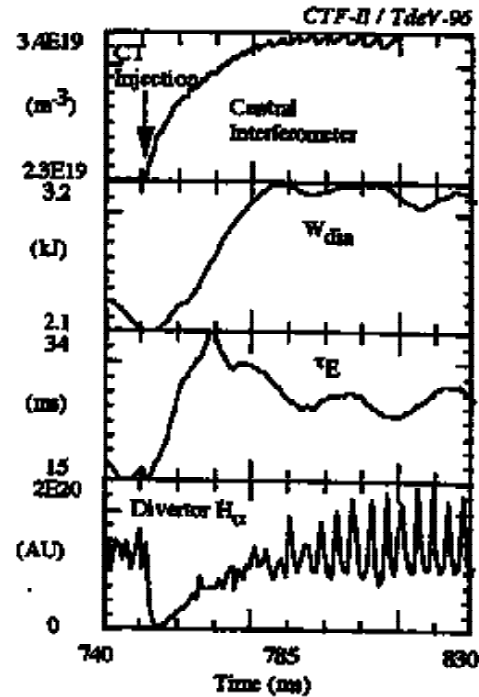
Figure 5: Example of improved confinement discharge from the CTF-II/TdsV96 run. B_T = 1.5 T, I_p = 170 kA, T_e(0) = 900 eV, single null discharge. Beyond t = 785 ms, the oscillation amplitude in the divertor H_{\alpha} signal increases.
