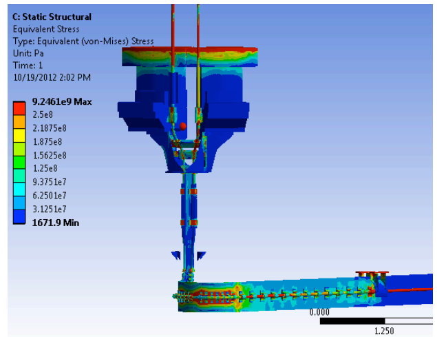
Figure 12. Stress in lower feeder parts (EOB)
