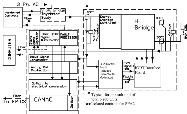
Figure 4 Block Diagram of controls
