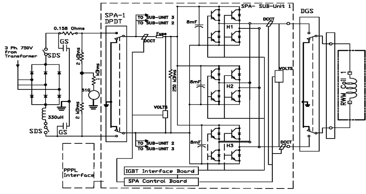
Figure 1 – RWM Power Loop
