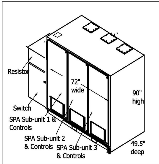
Figure -2: Outline of SPA-1
