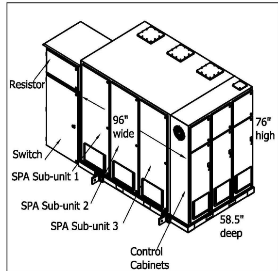
Figure -3: Outline of SPA-2
