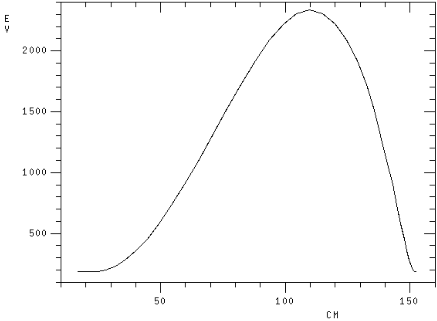
ELECTRON TEMPERATURE (TE) VS MIDPLANE RADII (RMAJM)
