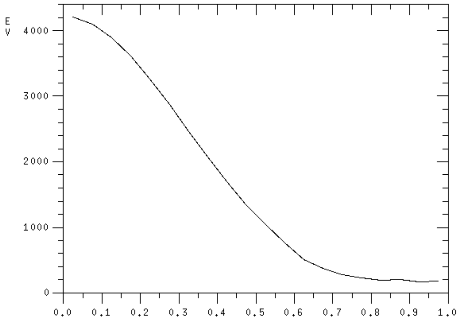
ION TEMPERATURE (TI) VS x"r/a" ctr (X)
