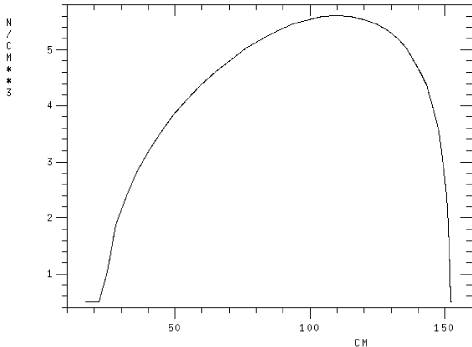
ELECTRON DENSITY (NE) VS MIDPLANE RADII (RMAJM)
