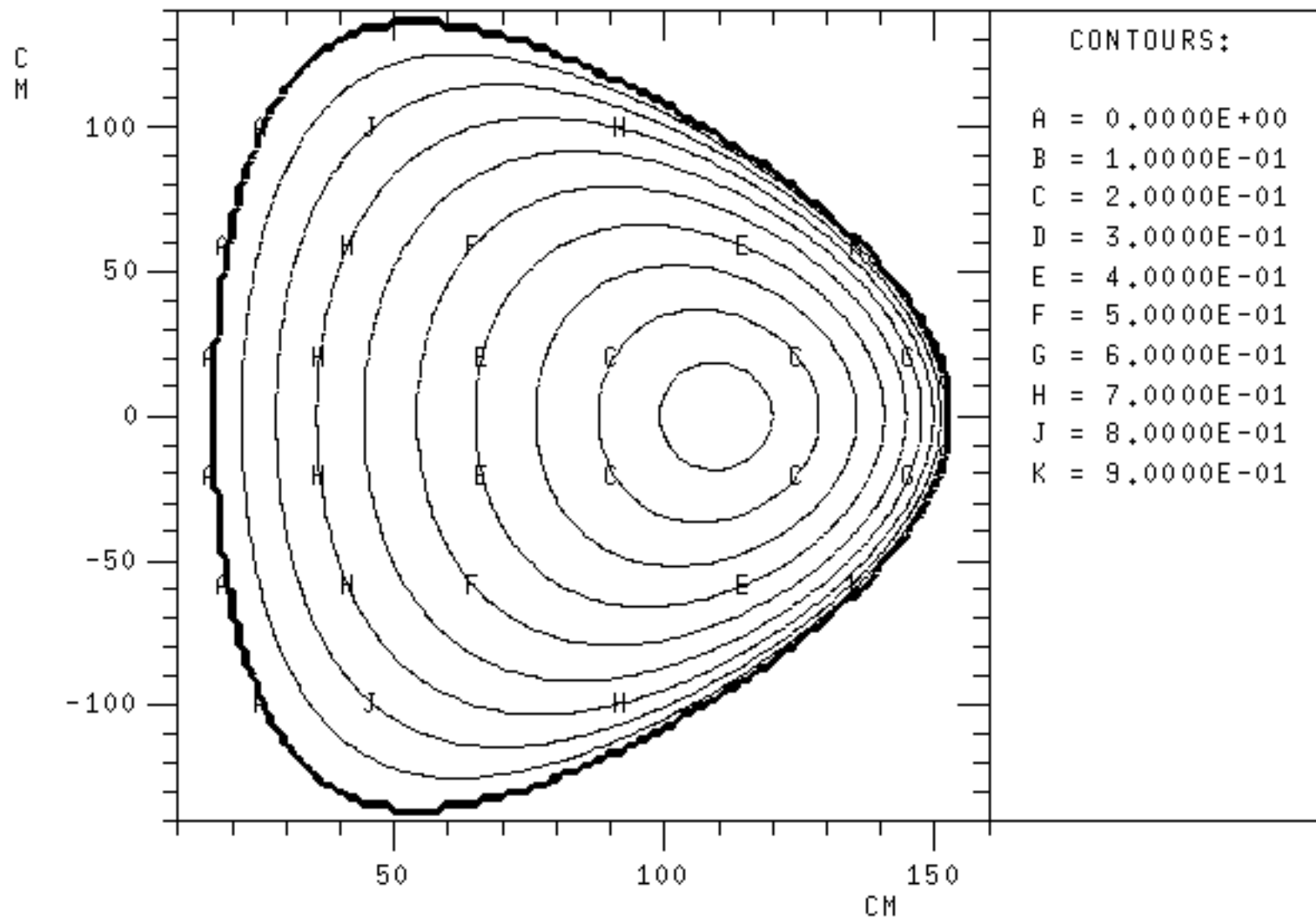
XI (sqrt norm tor. flux) CONTOUR PLOT VS R & Y
