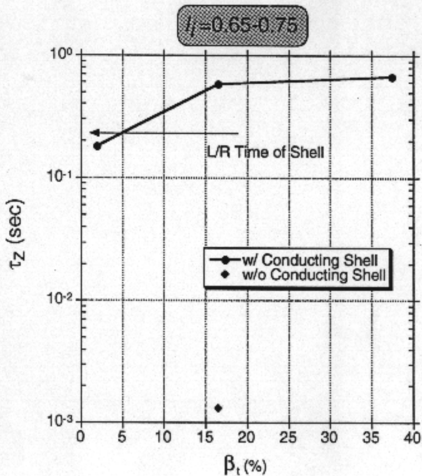
Vertical Stability Growth Times (1/2 in. Cu)
