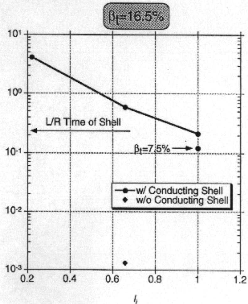
Vertical Stability Growth Times (1/2 in. Cu)
