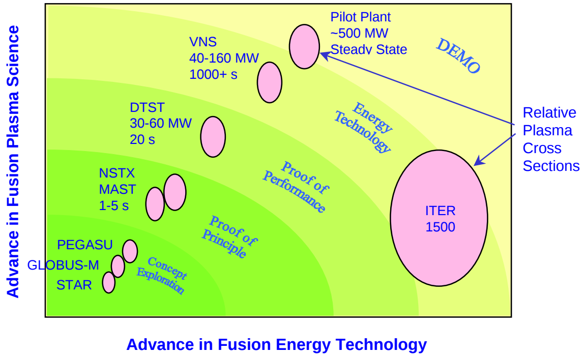
Figure 3. A pathway to fusion power utilizing the ST concept. Similar plasma dimensions are presently projected for the ST devices for Proof of Principle, Proof of Performance, Proof of Energy Technology, and the initial efforts for Power Demonstration.
