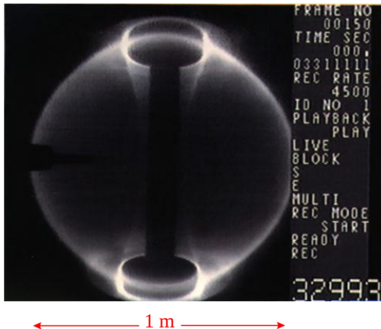
Figure 4. A high-speed video image of the small START plasma under NBI heating (courtesy of START team), indicating good plasma confinement and stability at high average toroidal beta ( \geq 30\% ).
