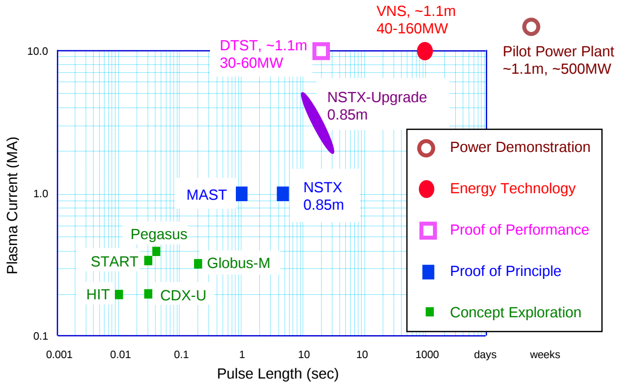
Figure 10. Plasma currents and pulse lengths of spherical torus experiments in advancing stages of development toward fusion power. Major radii and D-T burn powers are indicated for DTST, VNS, and Pilot Plant. NSTX and MAST will begin to prove the scientific principles of this pathway.
