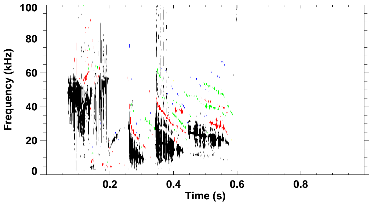
Shot 142184 \omega B(\omega) spectrum for toroidal mode number: 1 2 3 4 5
