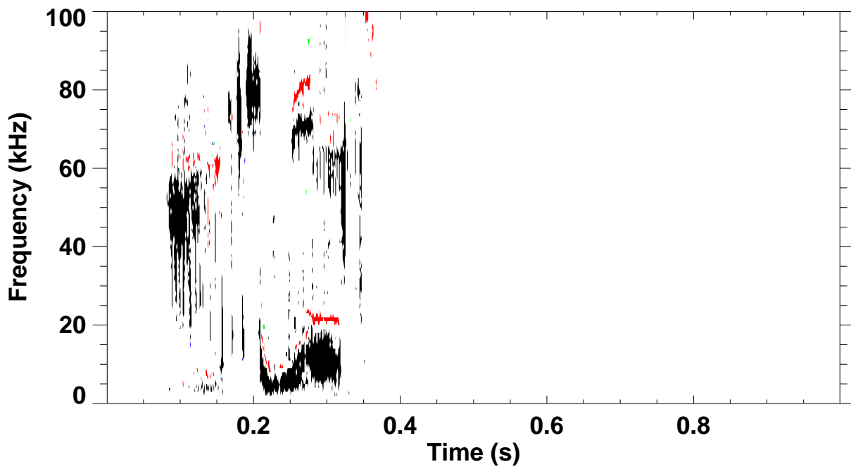
Shot 142459 \omega B(\omega) spectrum for toroidal mode number: 1 2 3 4 5
