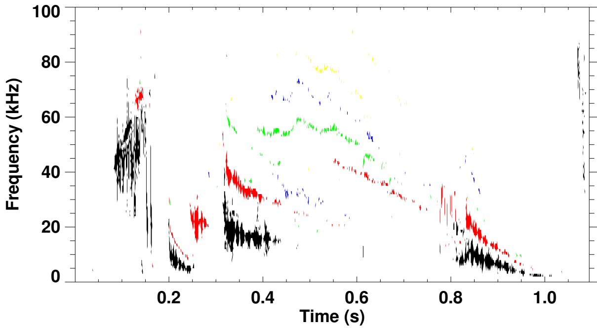
Shot 119087 \omega B(\omega) spectrum for toroidal mode number: 1 2 3 4 5
