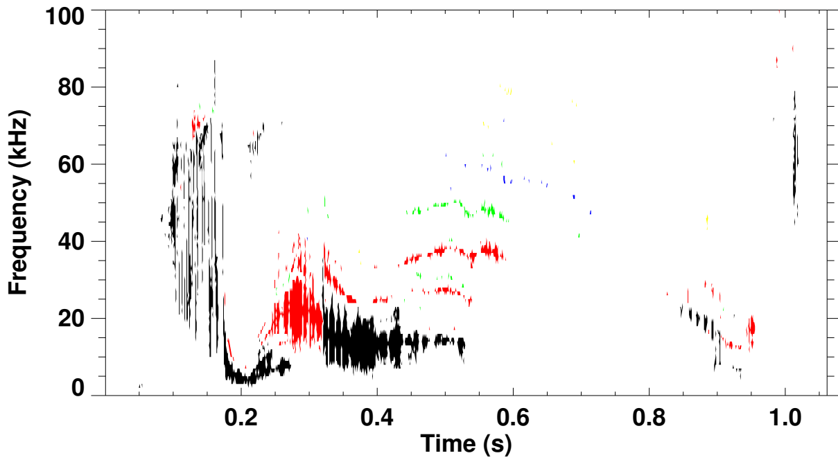
Shot 119673 \omega B(\omega) spectrum for toroidal mode number: 1 2 3 4 5
