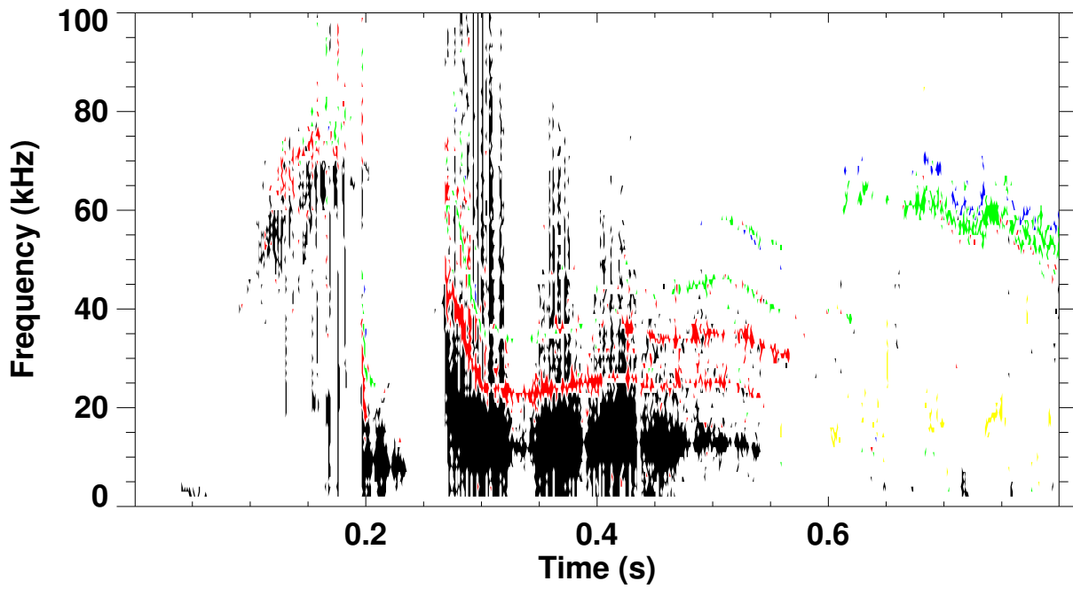
Shot 120041 \omega B(\omega) spectrum for toroidal mode number:
