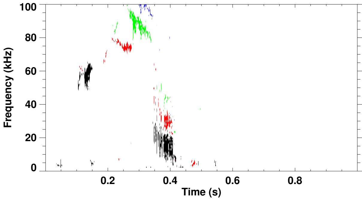
Shot 120142 \omega_B(\omega) spectrum for toroidal mode number: 1 2 3 4 5
