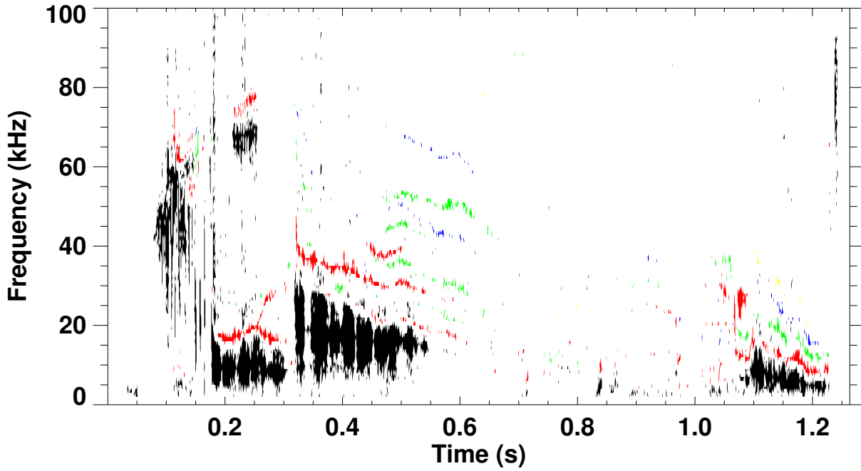
Shot 120157 \omega B(\omega) spectrum for toroidal mode number:
