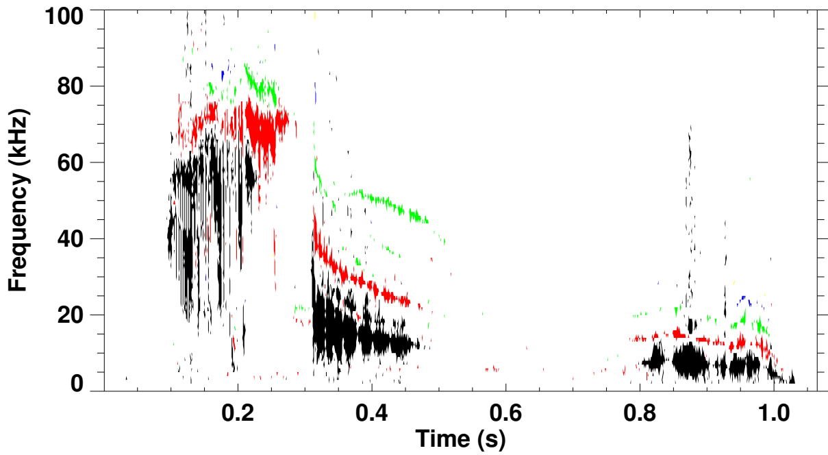
Shot 120986 \omega B(\omega) spectrum for toroidal mode number: 1 2 3 4 5
