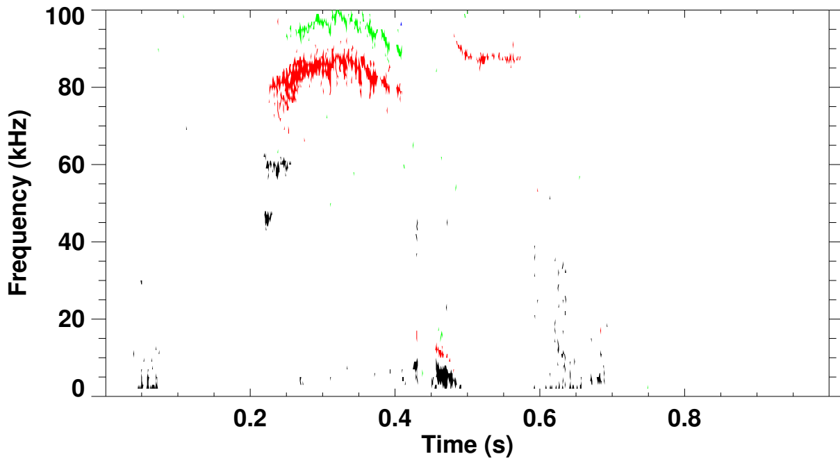
Shot 121549 \omega_B(\omega) spectrum for toroidal mode number: 1 2 3 4 5
