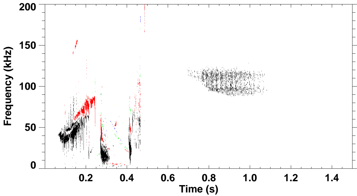
Shot 123016 \omega_B(\omega) spectrum for toroidal mode number: 1 2 3 4 5
