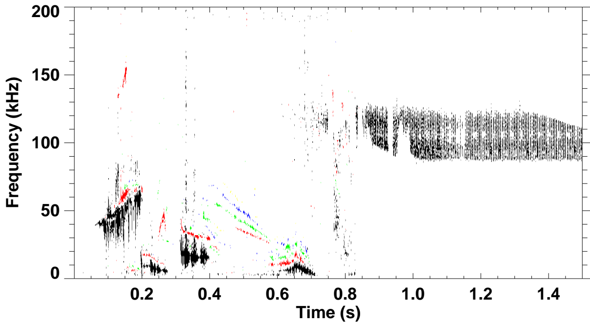
Shot 123118 \omega B(\omega) spectrum for toroidal mode number:
