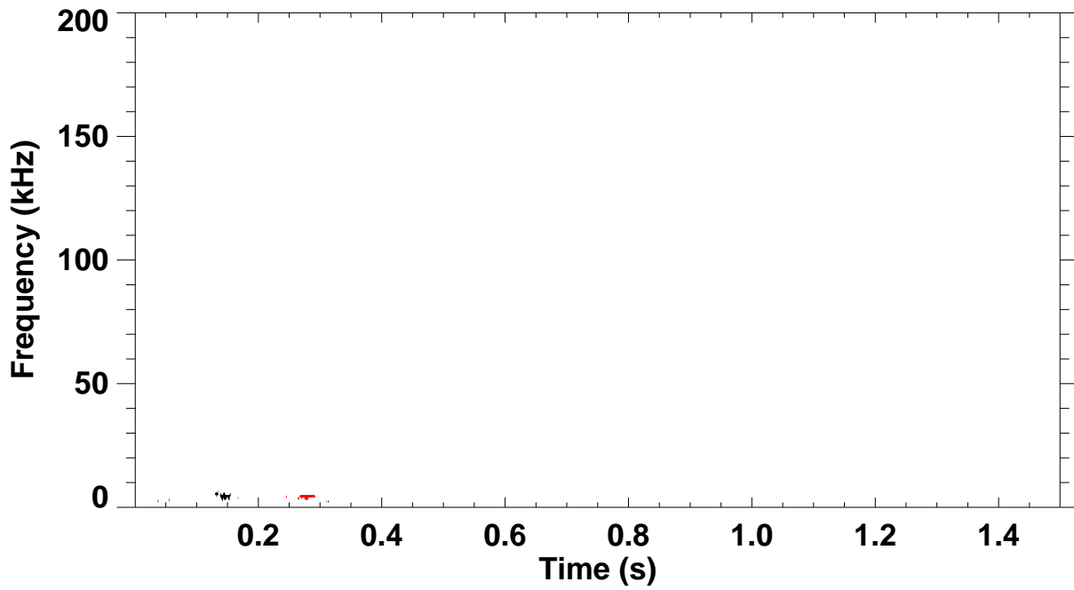
Shot 123678 \omega B(\omega) spectrum for toroidal mode number: 1 2 3 4 5
