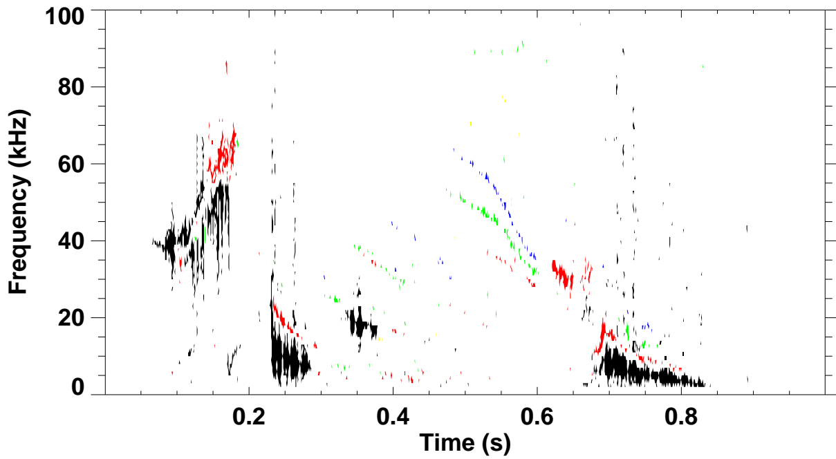
Shot 124011 \omega_B(\omega) spectrum for toroidal mode number: 1 2 3 4 5
