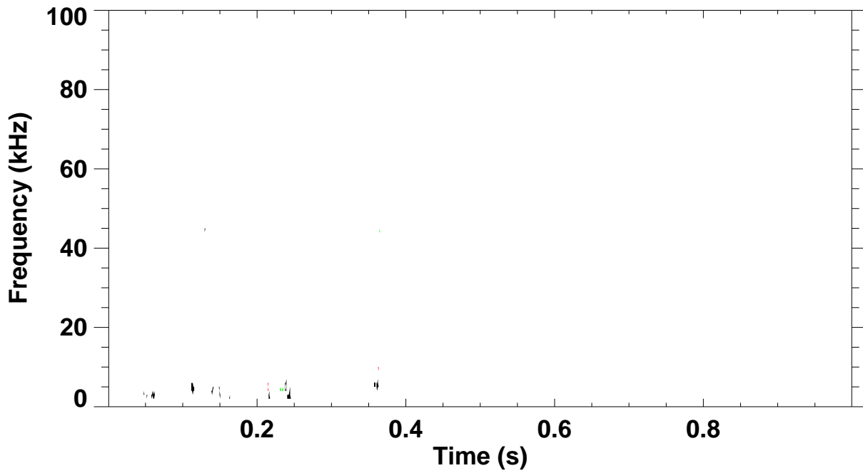
Shot 124059 \omega_B(\omega) spectrum for toroidal mode number: 1 2 3 4 5
