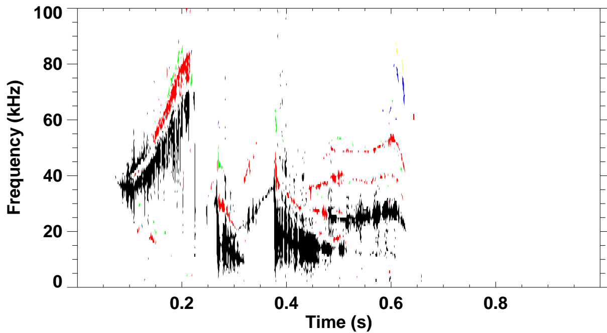
Shot 124294 \omega_B(\omega) spectrum for toroidal mode number: 1 2 3 4 5
