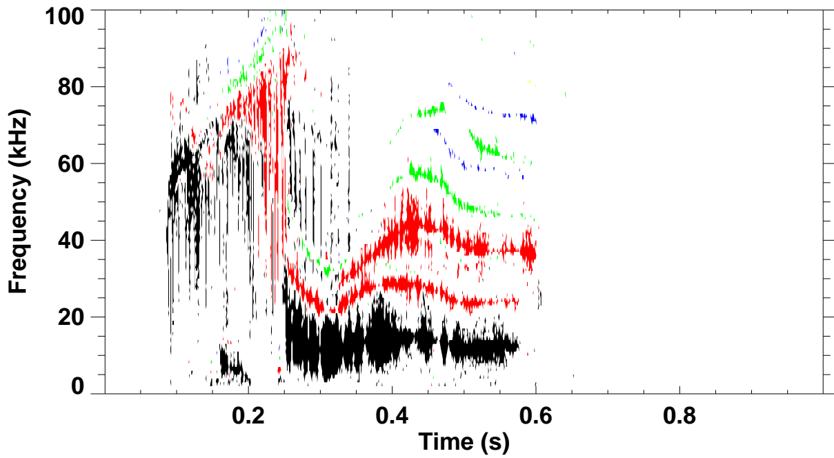
Shot 124412 \omega B(\omega) spectrum for toroidal mode number: 1 2 3 4 5
