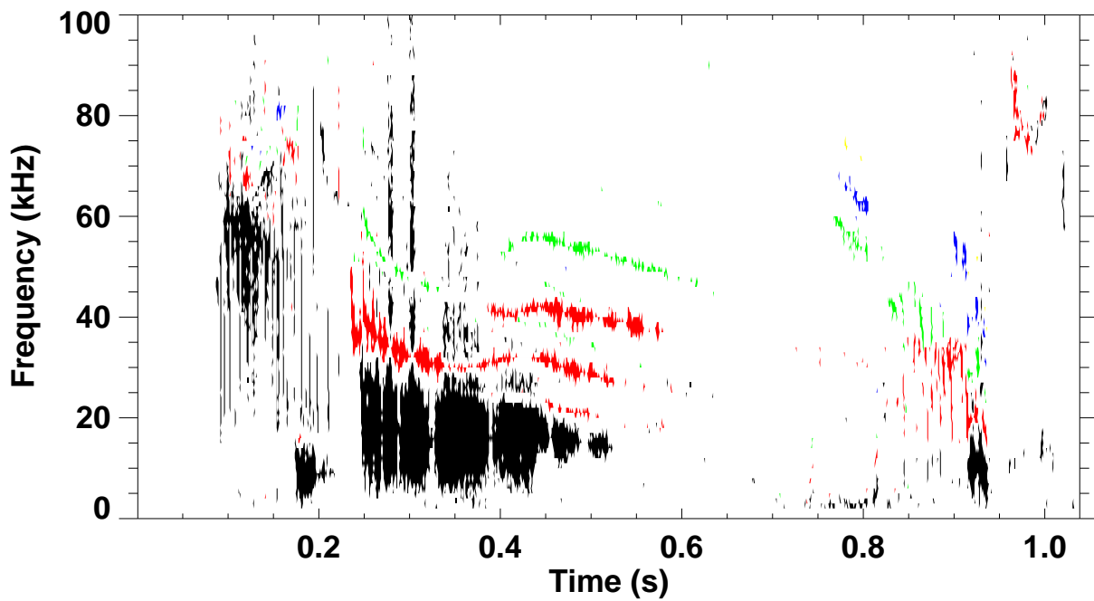
Shot 124426 \omega B(\omega) spectrum for toroidal mode number: 1 2 3 4 5
