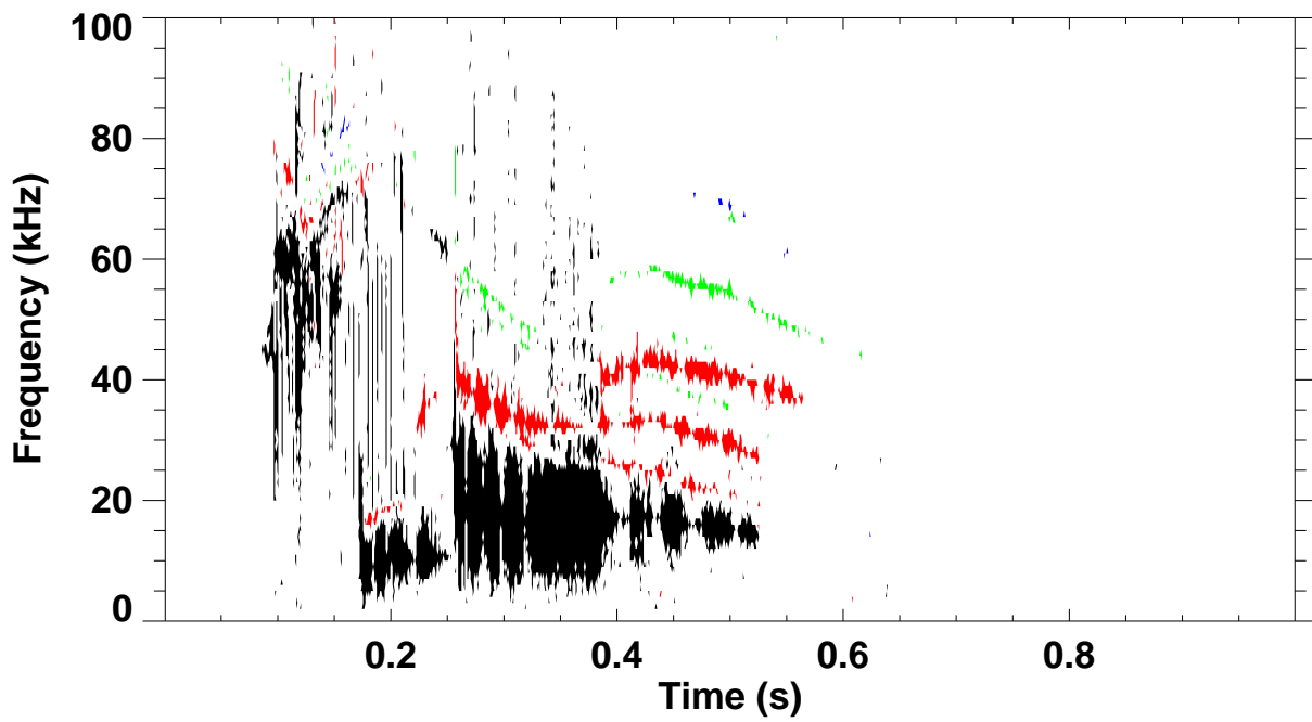
Shot 124436 \omega B(\omega) spectrum for toroidal mode number: 1 2 3 4 5
