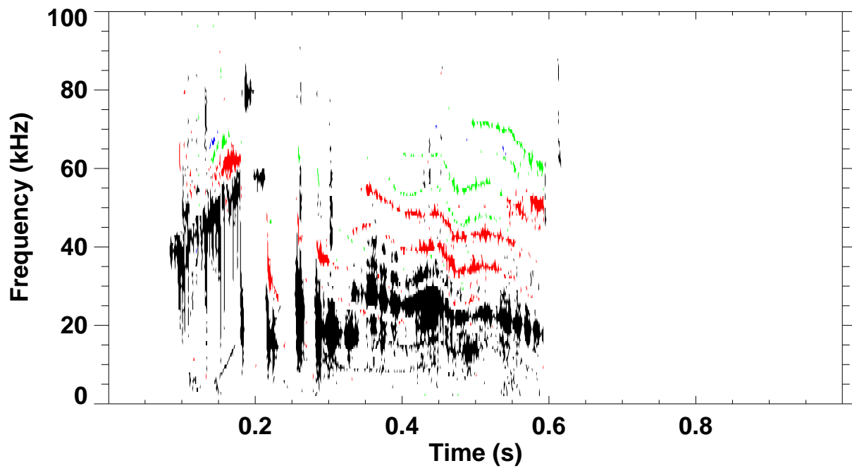
Shot 124576 \omega B(\omega) spectrum for toroidal mode number: 1 2 3 4 5
