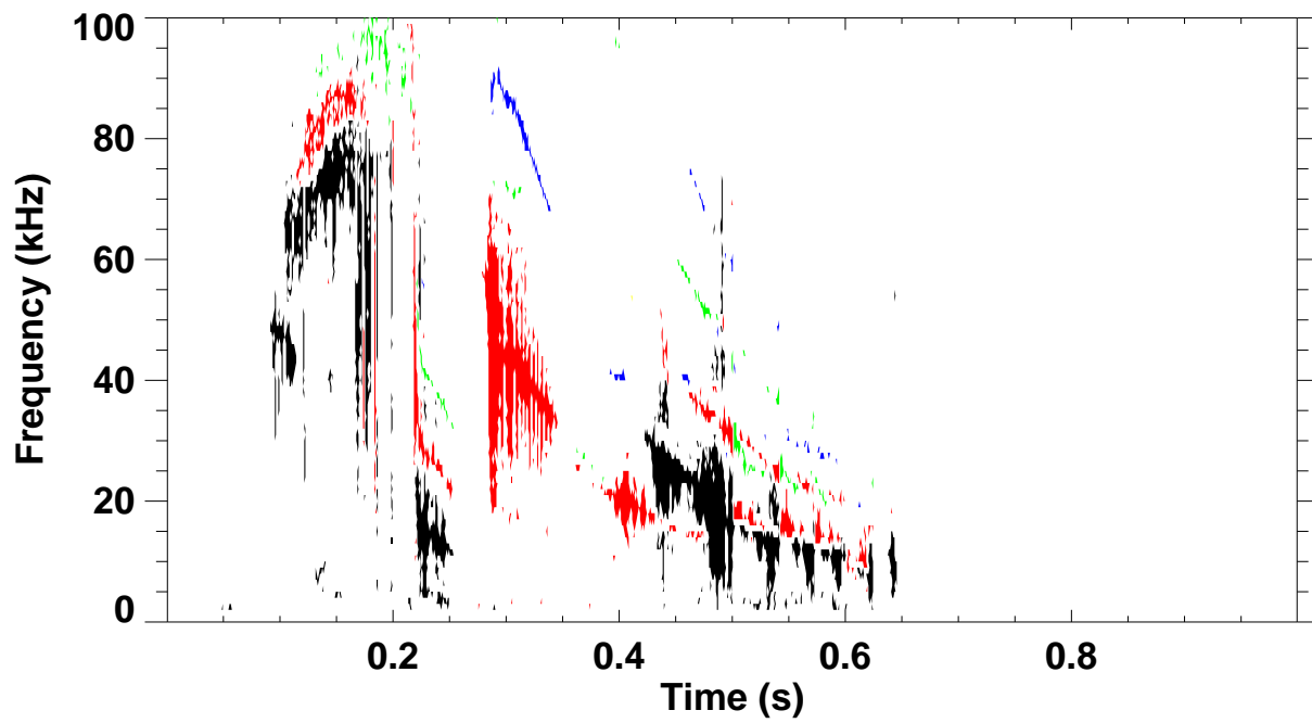
Shot 124670 \omega B(\omega) spectrum for toroidal mode number: 1 2 3 4 5
