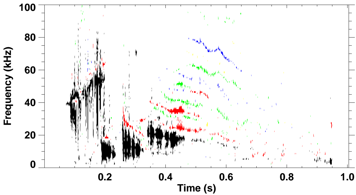
Shot 124707 \omega B(\omega) spectrum for toroidal mode number: 1 2 3 4 5
