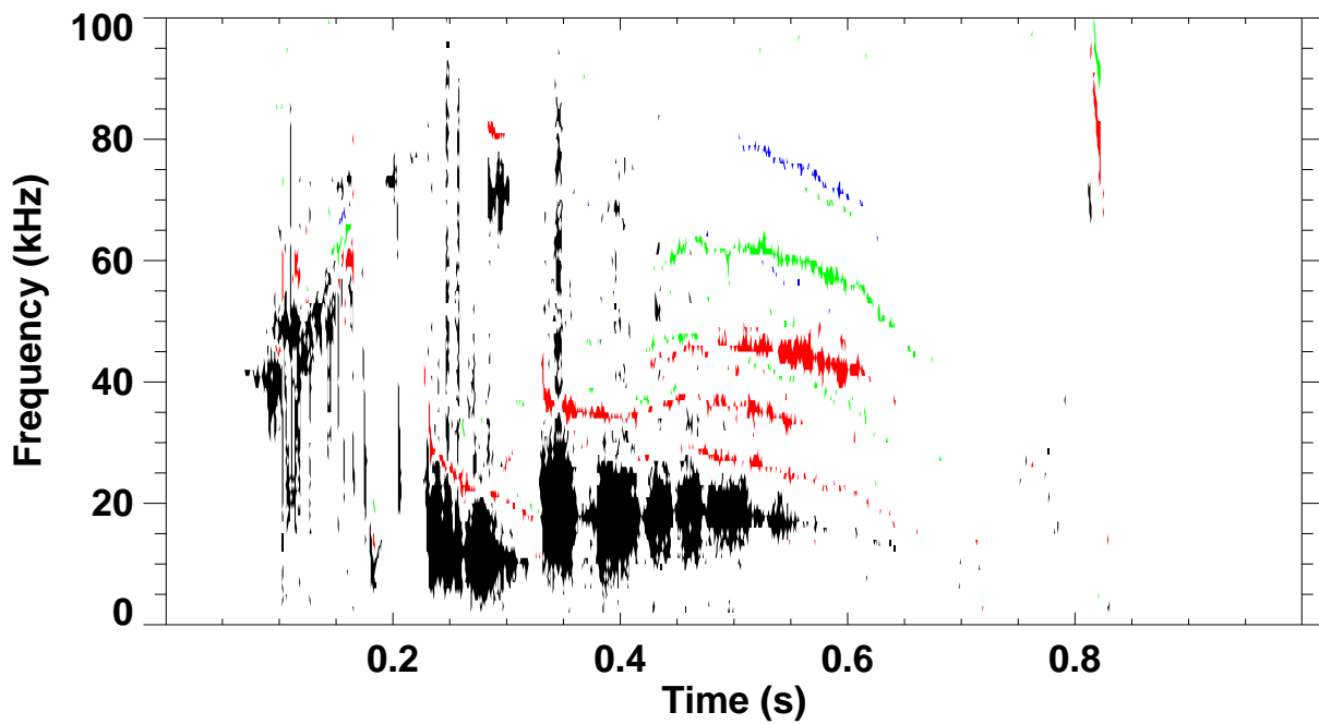
Shot 124755 \omega_B(\omega) spectrum for toroidal mode number: 1 2 3 4 5
