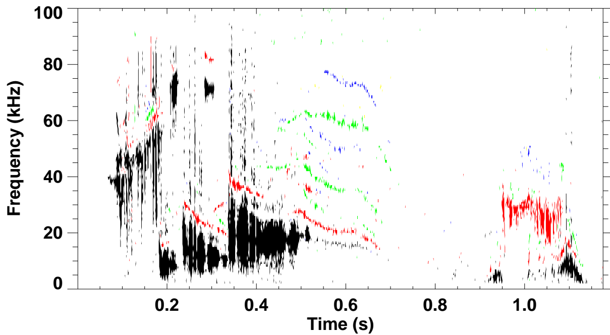
Shot 124757 \omega B(\omega) spectrum for toroidal mode number: 1 2 3 4 5
