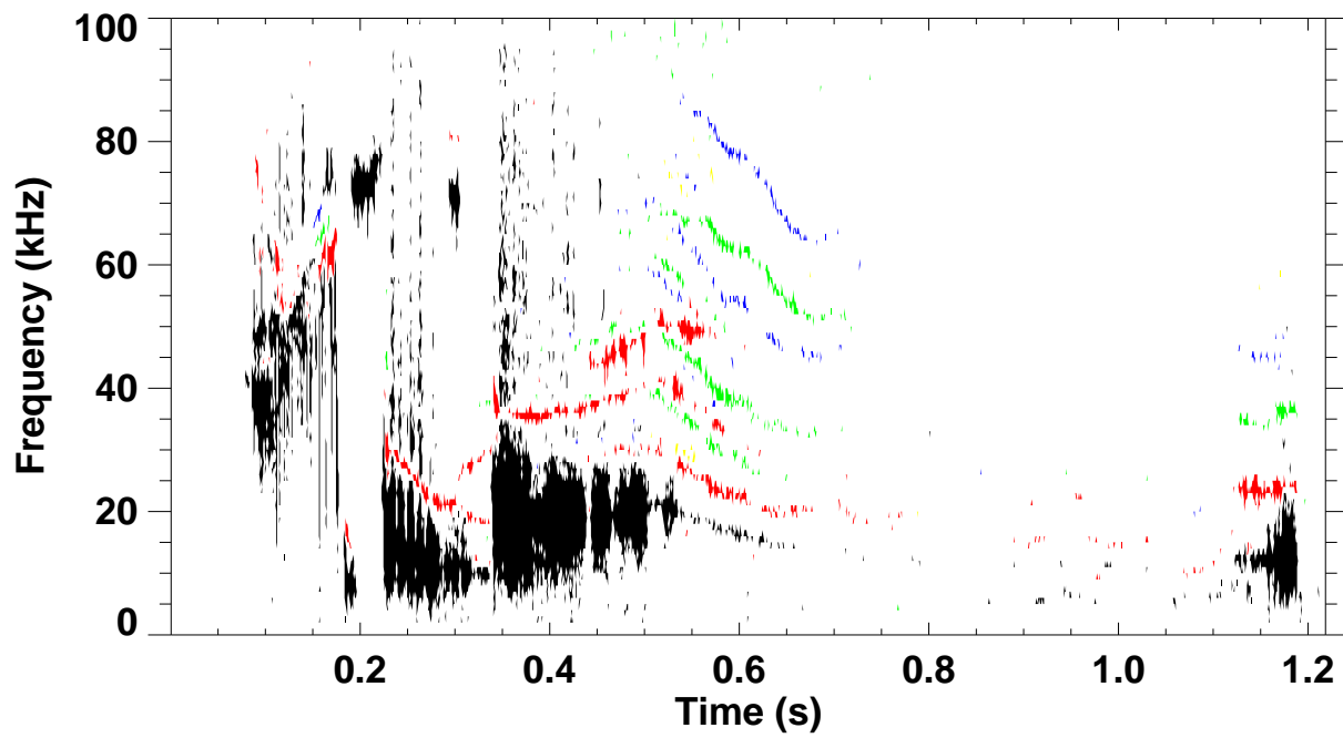
Shot 124802 \omega B(\omega) spectrum for toroidal mode number: 1 2 3 4 5
