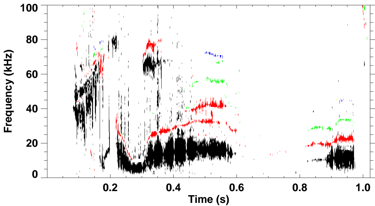
Shot 124819 \omega_B(\omega) spectrum for toroidal mode number: 1 2 3 4 5
