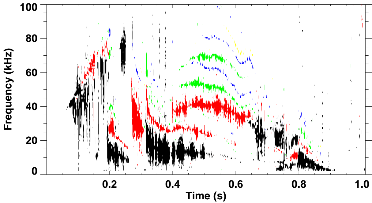
Shot 125280 \omega B(\omega) spectrum for toroidal mode number: 1 2 3 4 5
