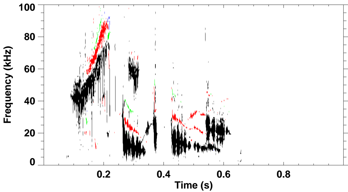
Shot 125290 \omega B(\omega) spectrum for toroidal mode number: 1 2 3 4 5
