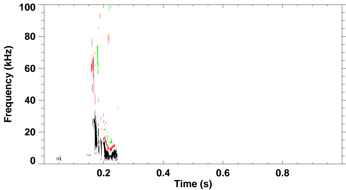
Shot 131775 \omega B(\omega) spectrum for toroidal mode number: 1 2 3 4 5
