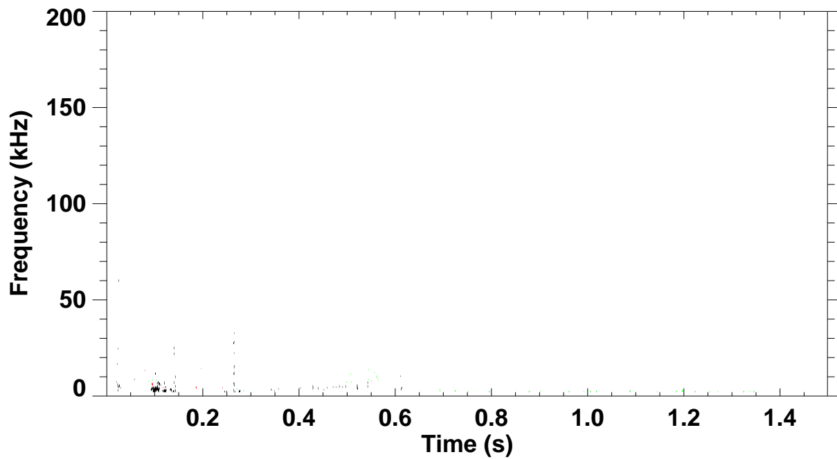
Shot 132122 \omega B(\omega) spectrum for toroidal mode number: 1 2 3 4 5
