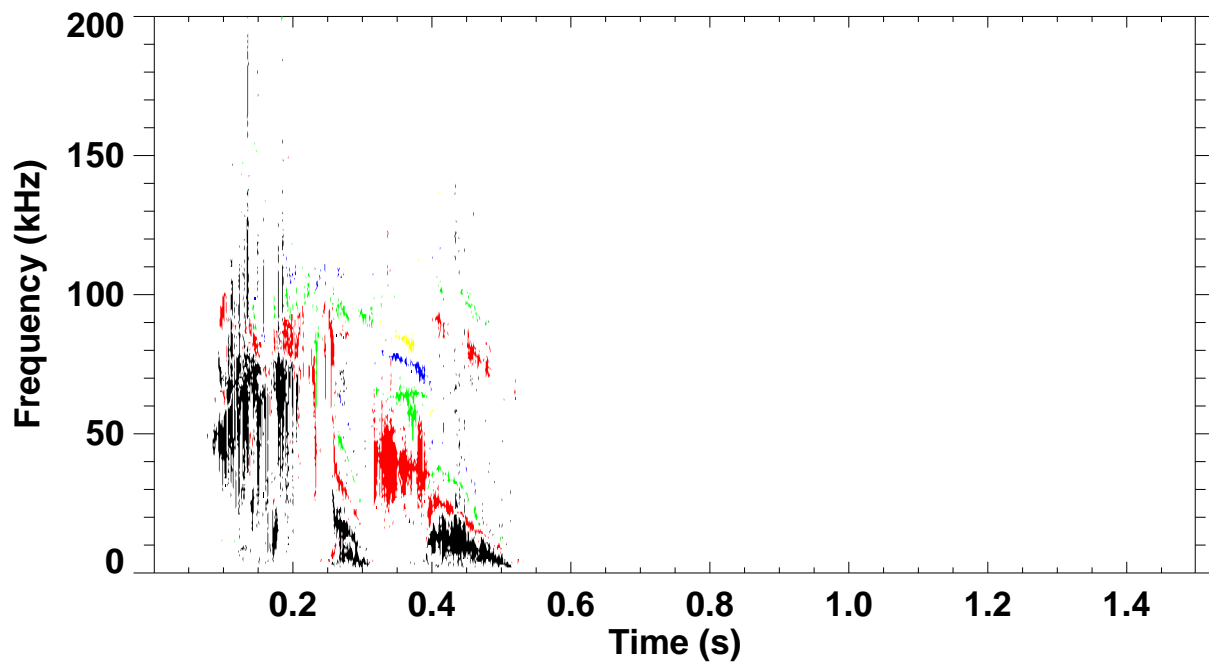
Shot 132167 \omega_B(\omega) spectrum for toroidal mode number: 1 2 3 4 5
