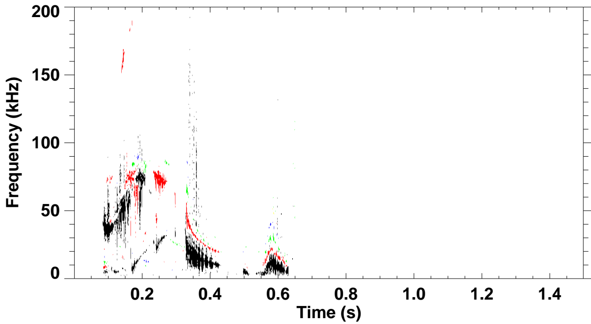
Shot 132184 \omega B(\omega) spectrum for toroidal mode number: 1 2 3 4 5
