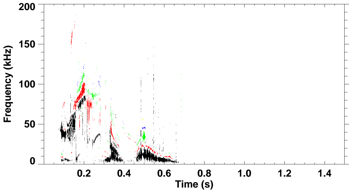
Shot 132185 \omega_B(\omega) spectrum for toroidal mode number: 1 2 3 4 5
